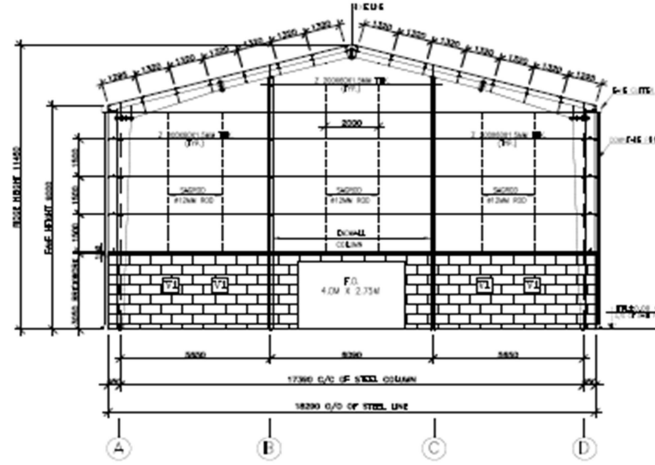
ENDWALL FRAMING ELEVATION (FOR FRAME LINES 5-8)
