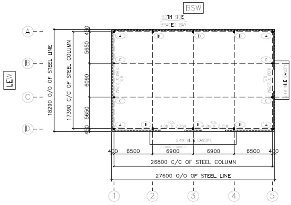
ANCHOR BOLT PLAN (F.F.L. ±0.00M I.V.L.)
