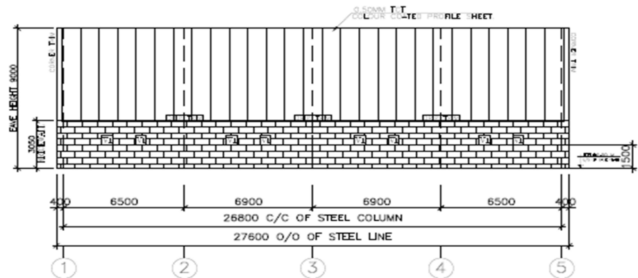
SIDEWALL SHEETING ELEVATION FOR FRAME LINE A
