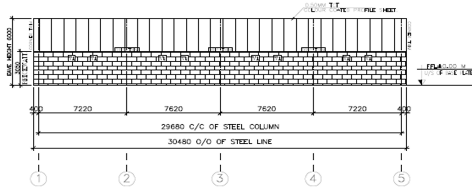
SIDEWALL SHEETING PLAN FOR FRAME LINE A
