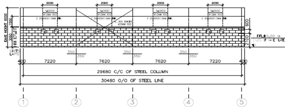
SIDEWALL FRAMING ELEVATION. FOR FRAME TYPE A
