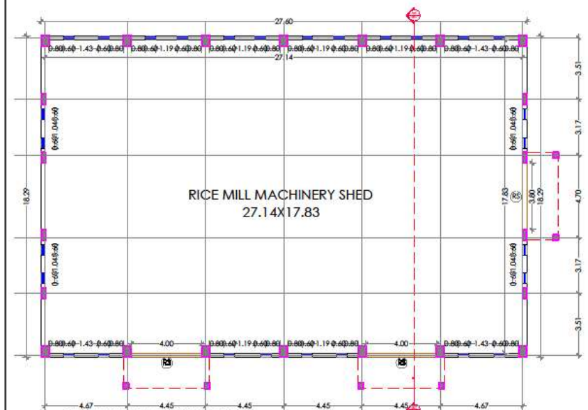
RICE MILL MACHINERY SHED DETAIL FLOOR PLAN
