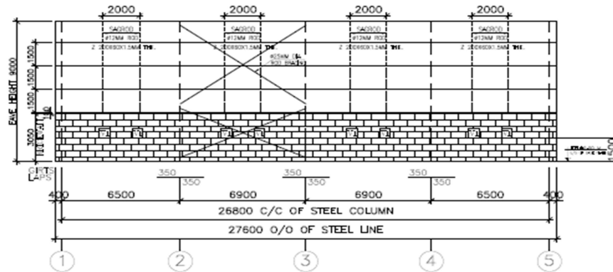
SIDEWALL FRAMING ELEVATION FOR FRAME TYPE A
