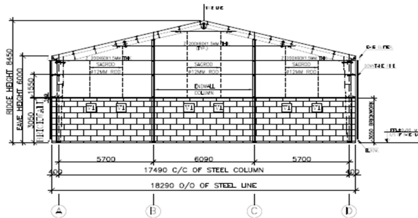
ENDWALL FRAMING ELEVATION (FOR FRAME LINE 5)
