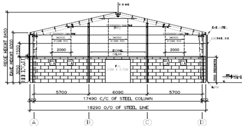
ENDWALL FRAMING ELEVATION (FOR FRAME LINE 1)
