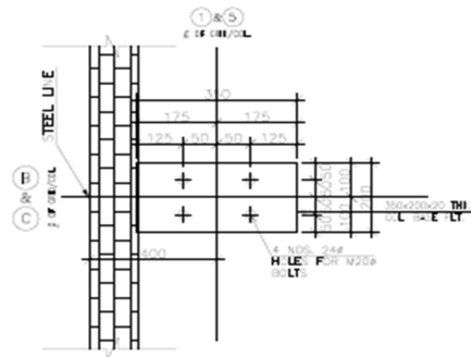
DETAIL C. (04 Nos. REOD.)
