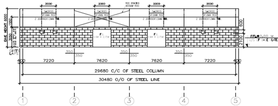
SIDEWALL FRAMING ELEVATION. FOR FRAME TYPE D
