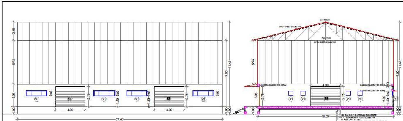
RICE MILL MACHINERY SHED FRONT ELEVATION
