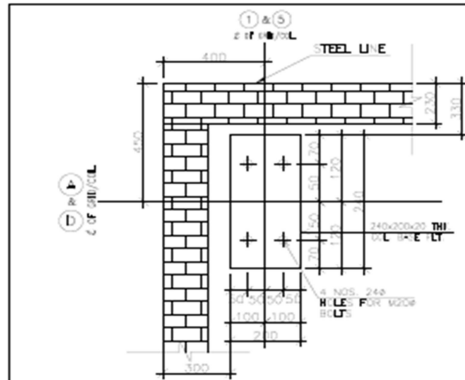
DETAIL A (4 Nos. REOD.)
