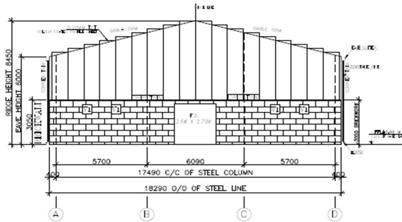
ENDWALL SHEETING ELEVATION (FOR FRAME LINE 1)
