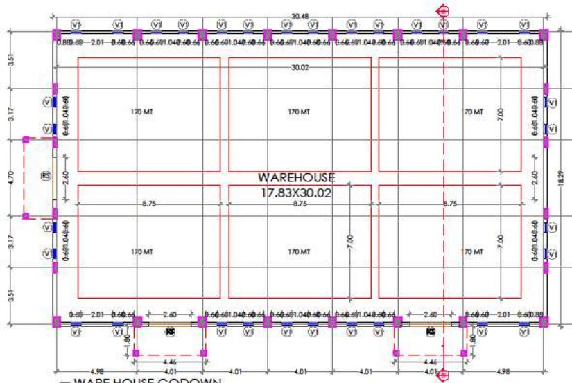
WARE HOUSE GODOWN DETAIL FLOOR PLAN
