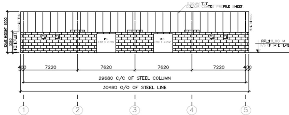
SIDEWALL SHEETING PLAN FOR FRAME LINE D
