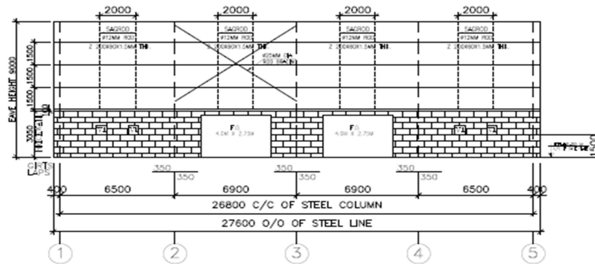
SIDEWALL FRAMING ELEVATION FOR FRAME TYPE D
