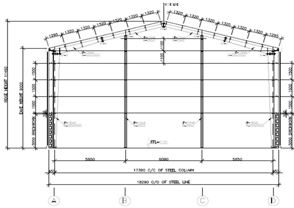
RIGID FRAME CROSS SECTION (FOR FRAME LINES 1&5.)
