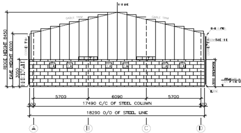
ENDWALL SHEETING ELEVATION (FOR FRAME LINE 5)
