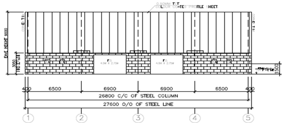
SIDEWALL SHEETING ELEVATION FOR FRAME LINE D
